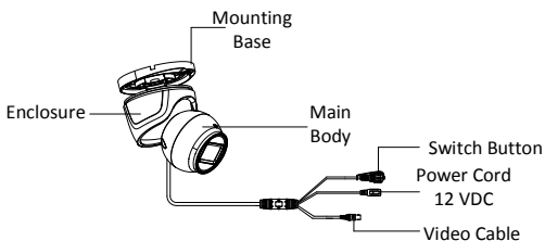
Figure 1-2 Overview of Type II Camera
