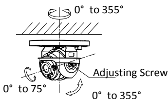
Figure 2-14 Type III Camera 3-Axis Adjustment
