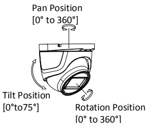
Figure 2-10 3-axis Adjustment
