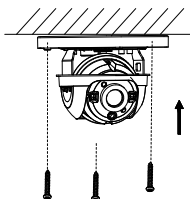
Figure 2-13 Install the Mounting Base
