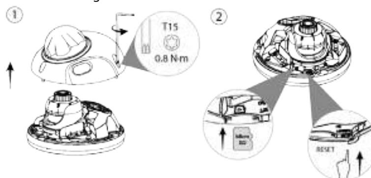
Figure 3-4 Install the SD card
