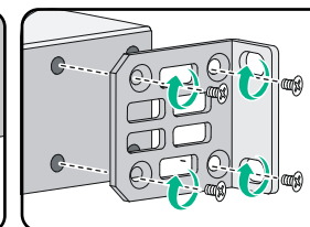
Attach a Type A front mounting bracket near the power module side
