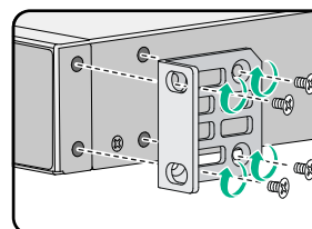
Attach a Type A front mounting bracket near the port side
