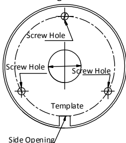
Figure 2-1 Drill Template
