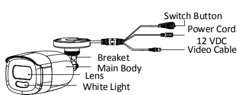
Figure 1-2 Overview of Type II Camera Installation
