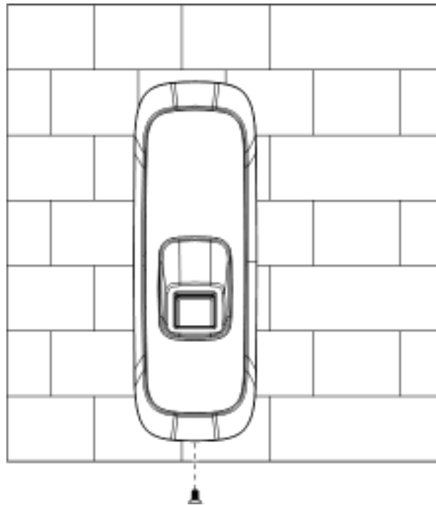
Figure 2-2 Drill holes (unit:mm[inch])
