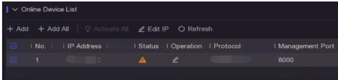
Figure 6-12 Online Device
