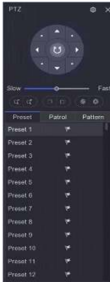
Figure 2-3 PTZ Settings
