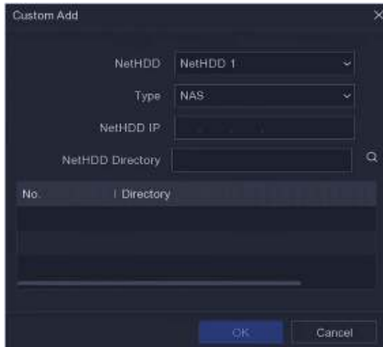
Figure 5-13 Add NetHDD
