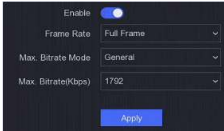
Figure 6-3 Channel-Zero
