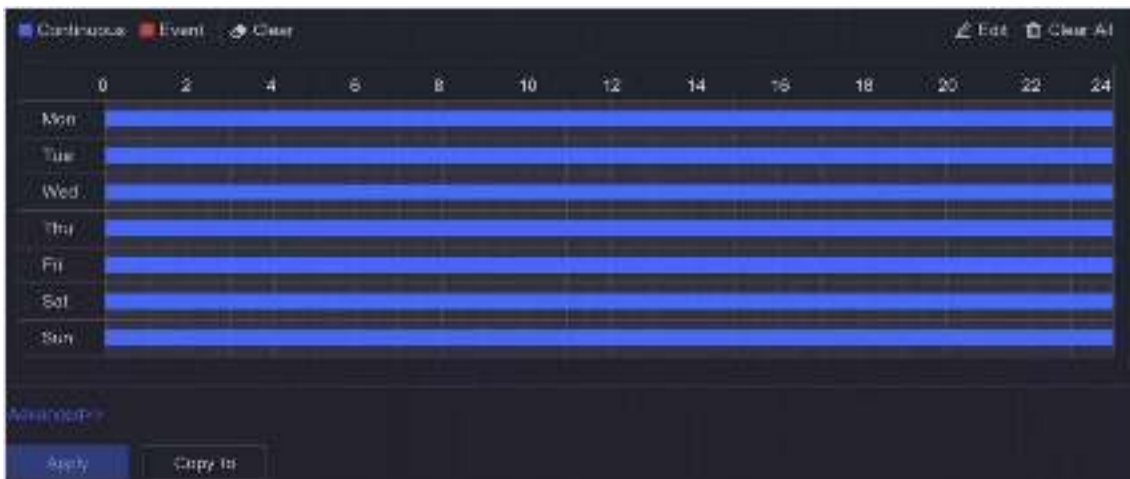
Figure 6-26 Recording Schedule
