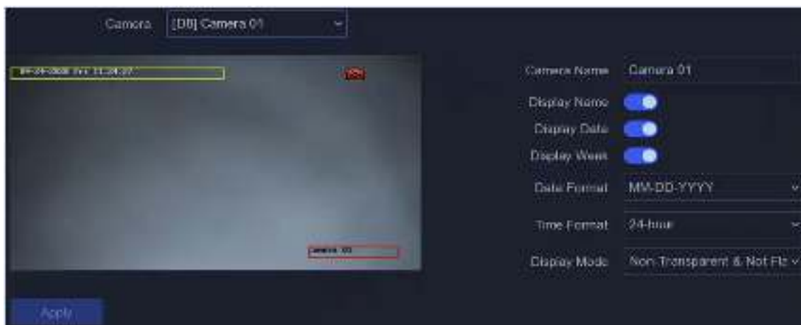
Figure 5-11 OSD
