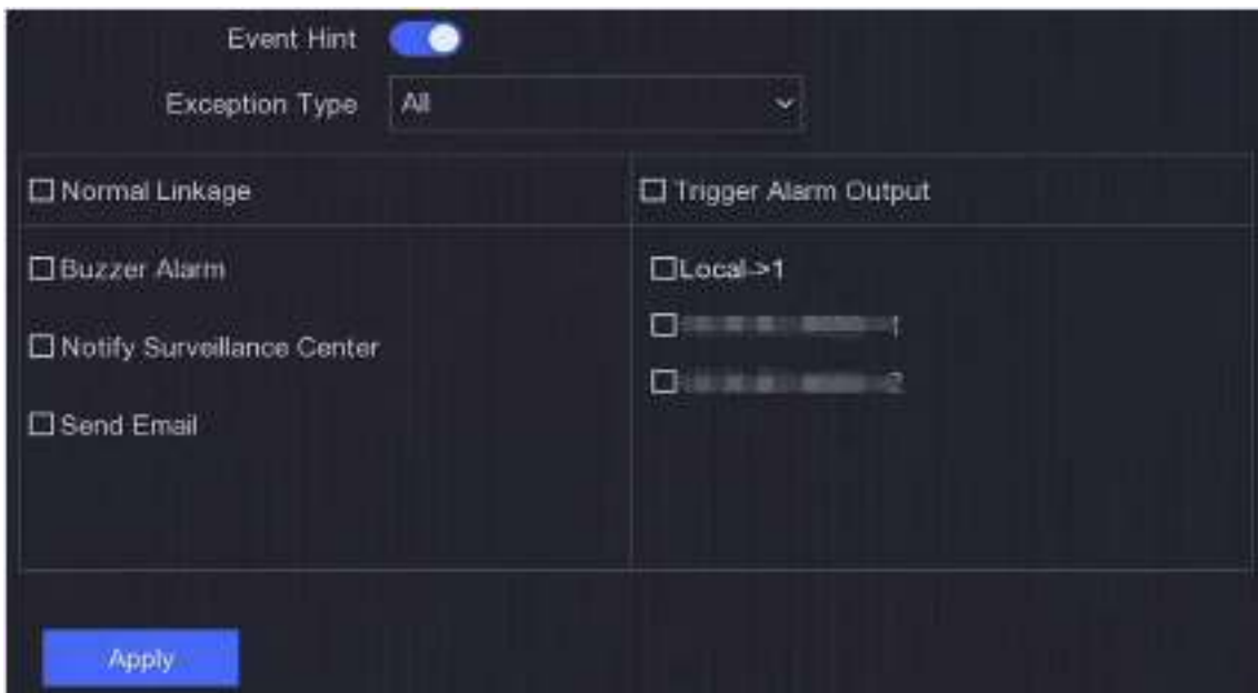
Figure 5-3 Exceptions
