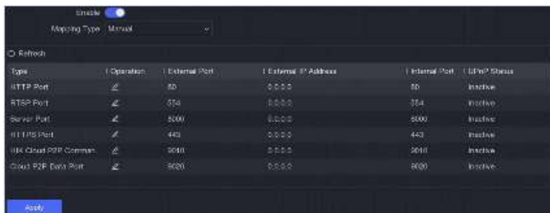
Figure 6-5 NAT
