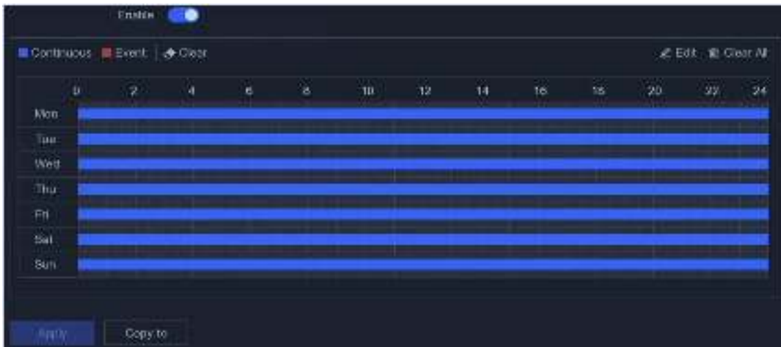
Figure 5-14 Recording Schedule
