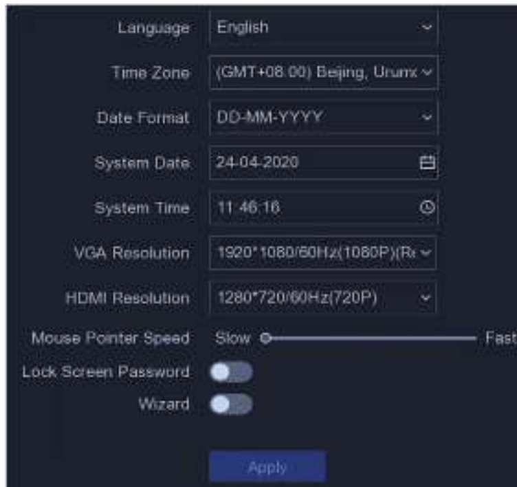
Figure 6-1 Basic Settings
