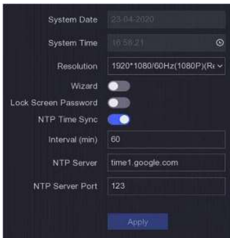
Figure 5-1 General Settings
