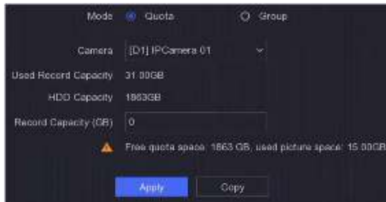
Figure 6-30 Quota
