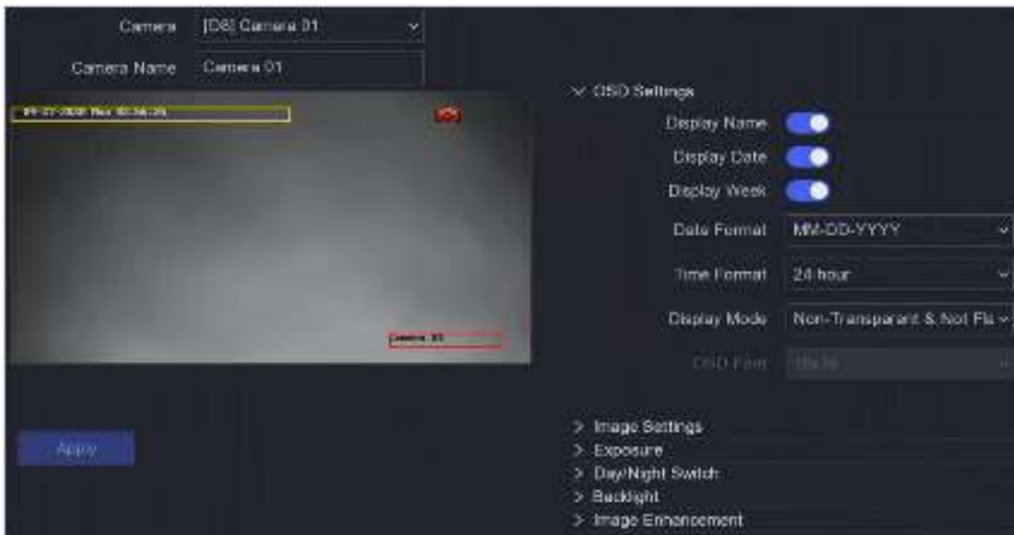
Figure 6-14 OSD
