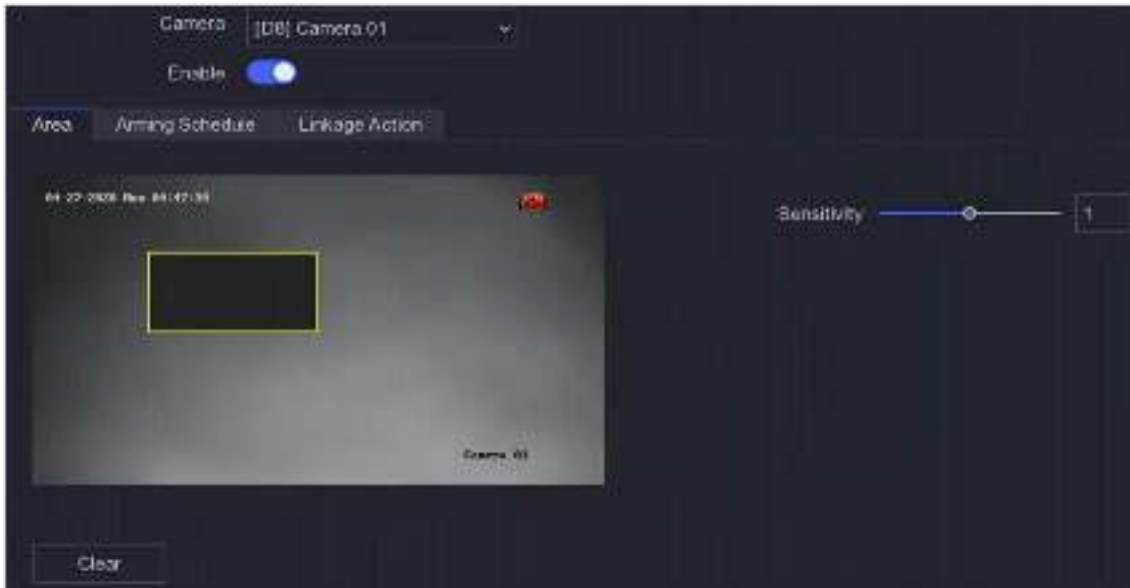
Figure 6-16 Video Tampering
