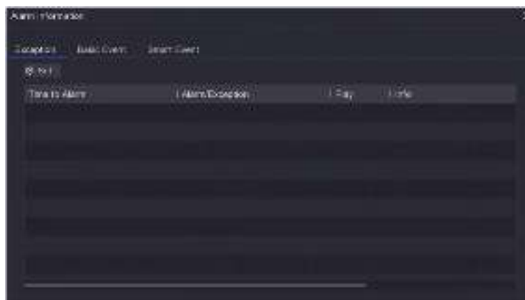
Figure 8-1 Alarm Center
