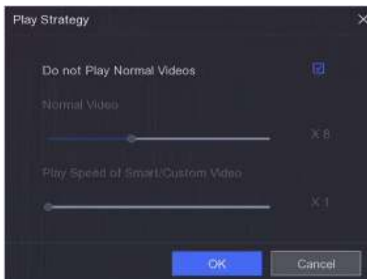
Figure 3-5 Play Strategy
