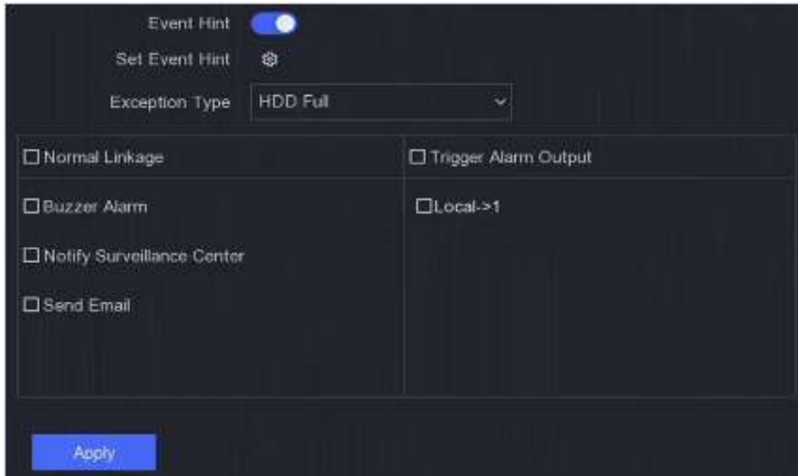
Figure 6-21 Exceptions
