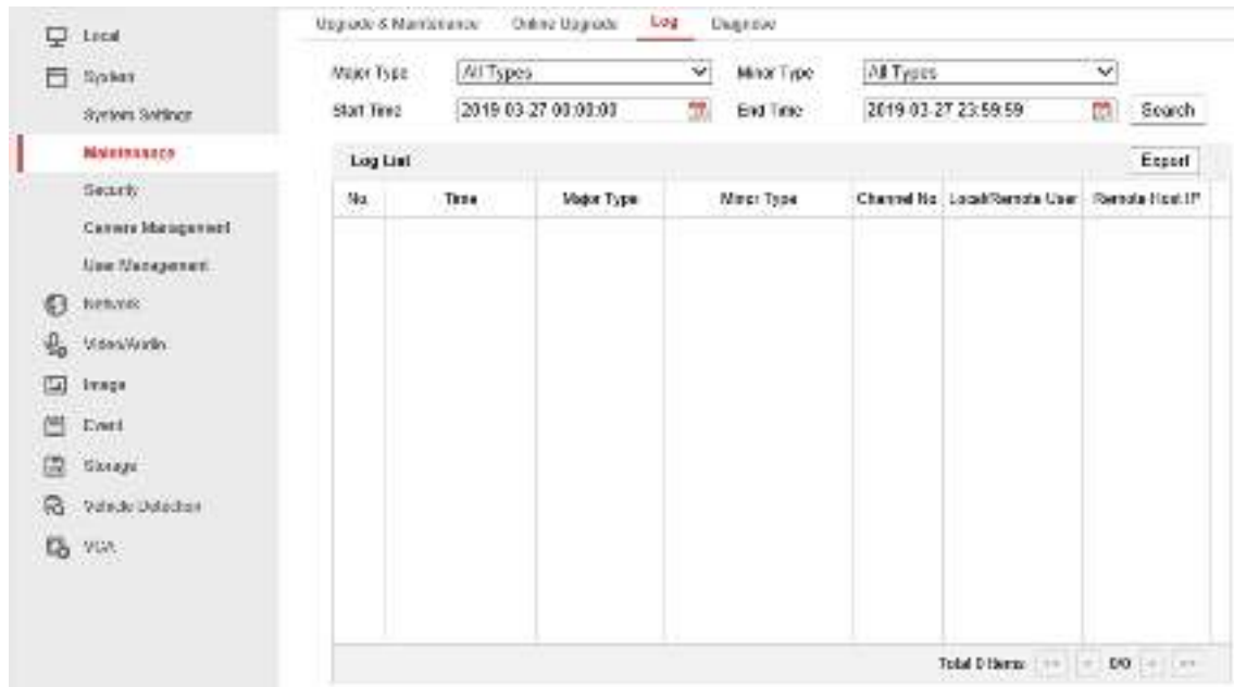
Figure 9-5 Log
