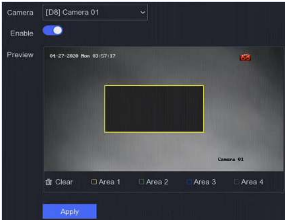
Figure 6-15 Privacy Mask
