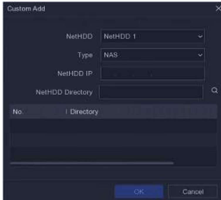
Figure 6-28 Add NetHDD
