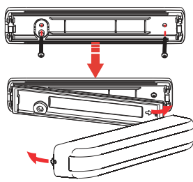
Mounting with the general mounting plate.
