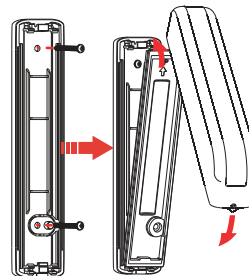
Mounting with the general mounting plate.
