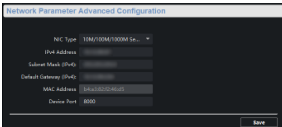
Figure 5-1 Network Configuration
