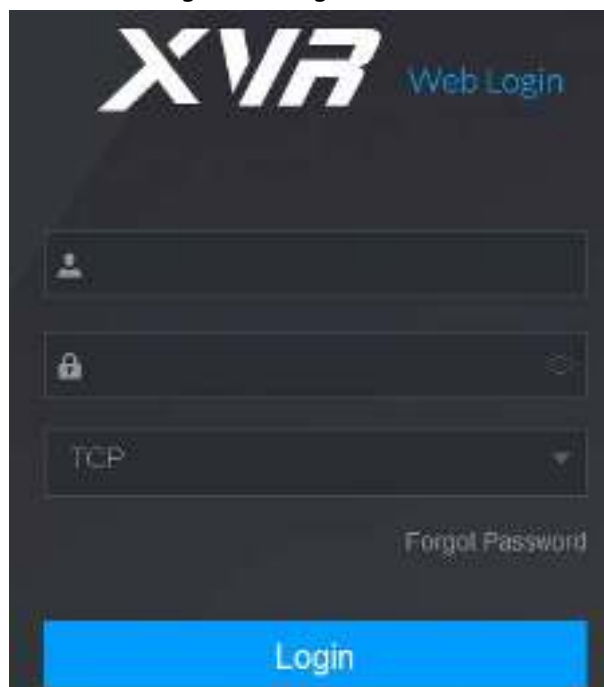
Figure 2-1 Login
